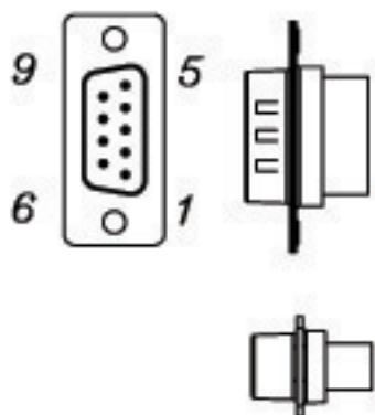
DB9 MALE CRIMP TYPE
